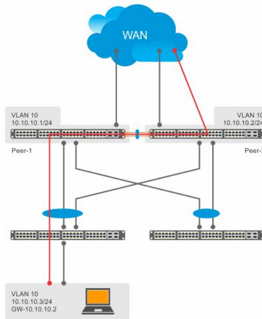
Figure 138. Packets without peer routing enabled
