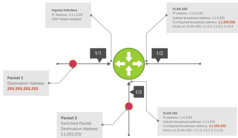
Figure 54. UDP Helper with Configured Broadcast Addresses
