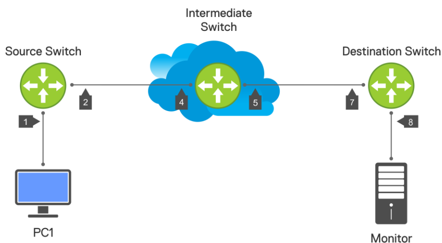
Figure 103. RPM Configuration
