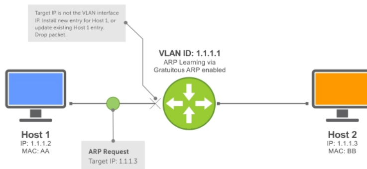
Figure 50. ARP Learning via ARP Request with ARP Learning via Gratuitous ARP Enabled
