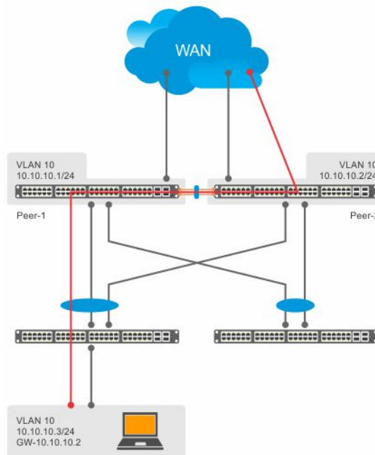
Figure 143. Packets without peer routing enabled
