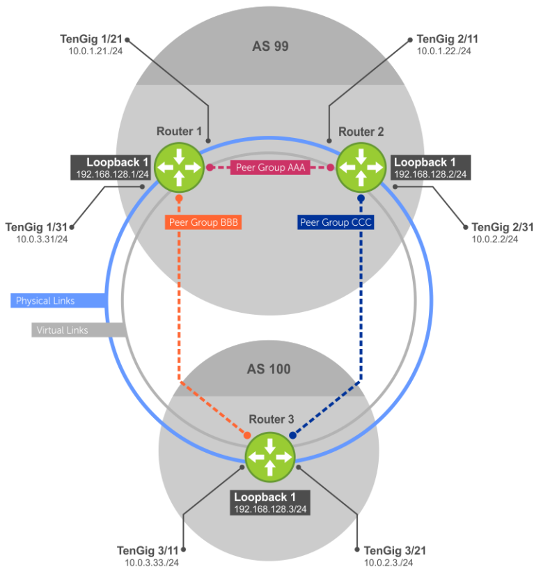
Figure 24. BGP peer group example configurations
