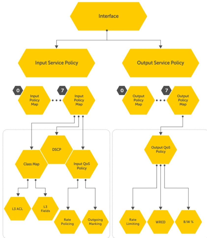
Figure 115. Constructing Policy-Based QoS Configurations
