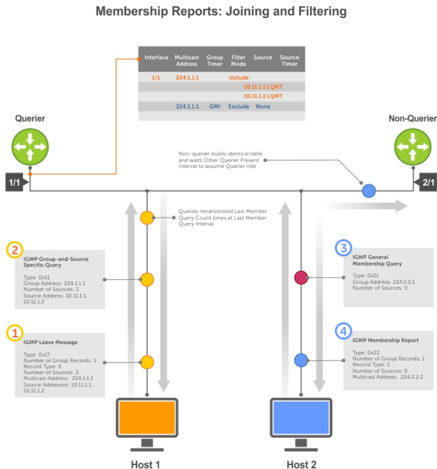
Figure 38. Membership Queries: Leaving and Staying
