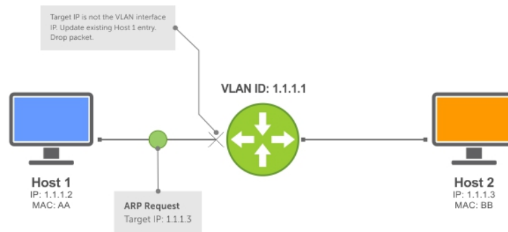
Figure 41. ARP Learning via ARP Request
