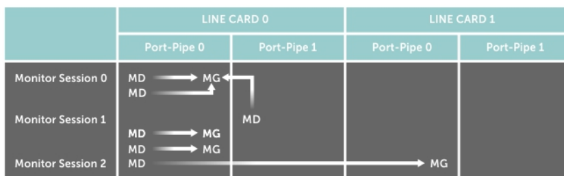
Figure 94. Port Monitoring Configurations
