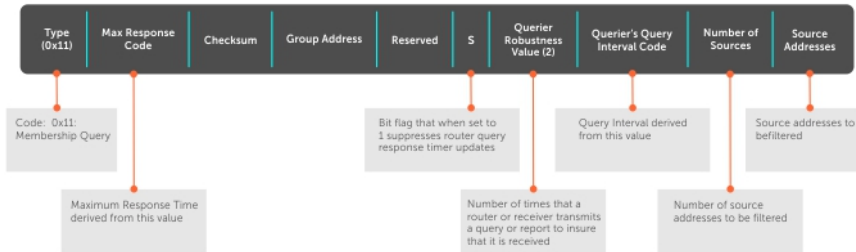
Figure 44. IGMP Version 3 Packet Structure
