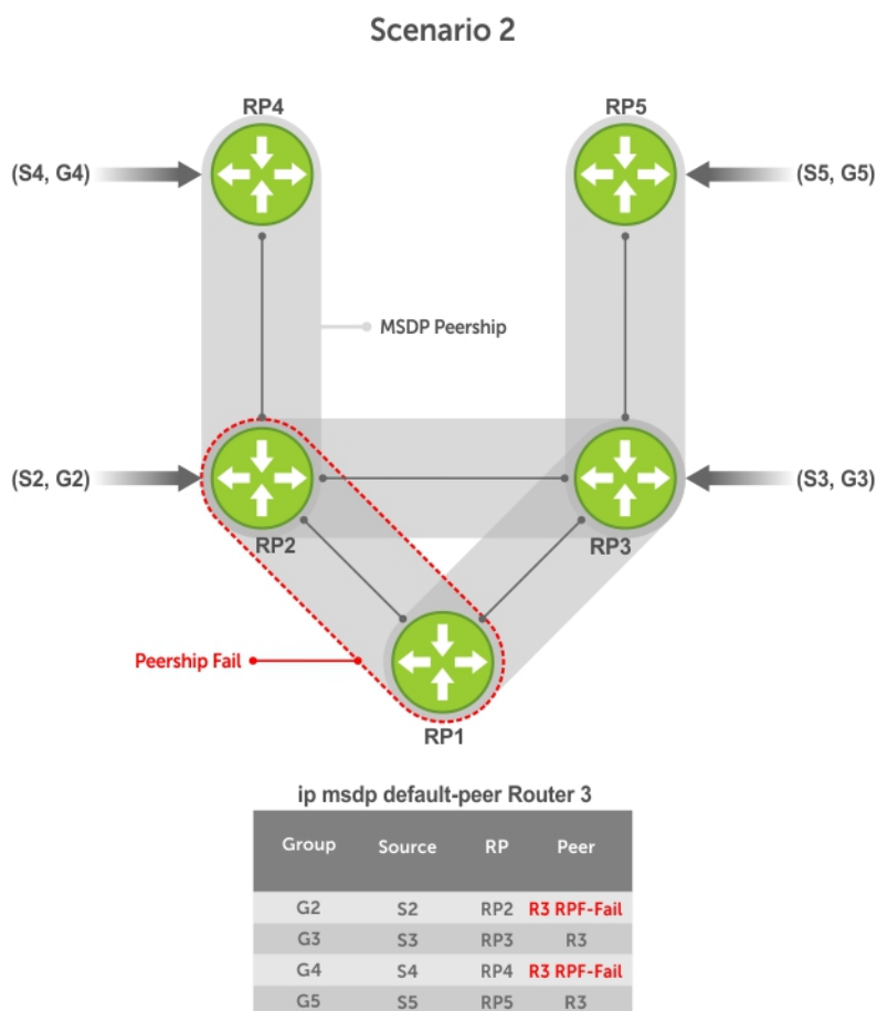
Figure 87. MSDP Default Peer, Scenario 2
