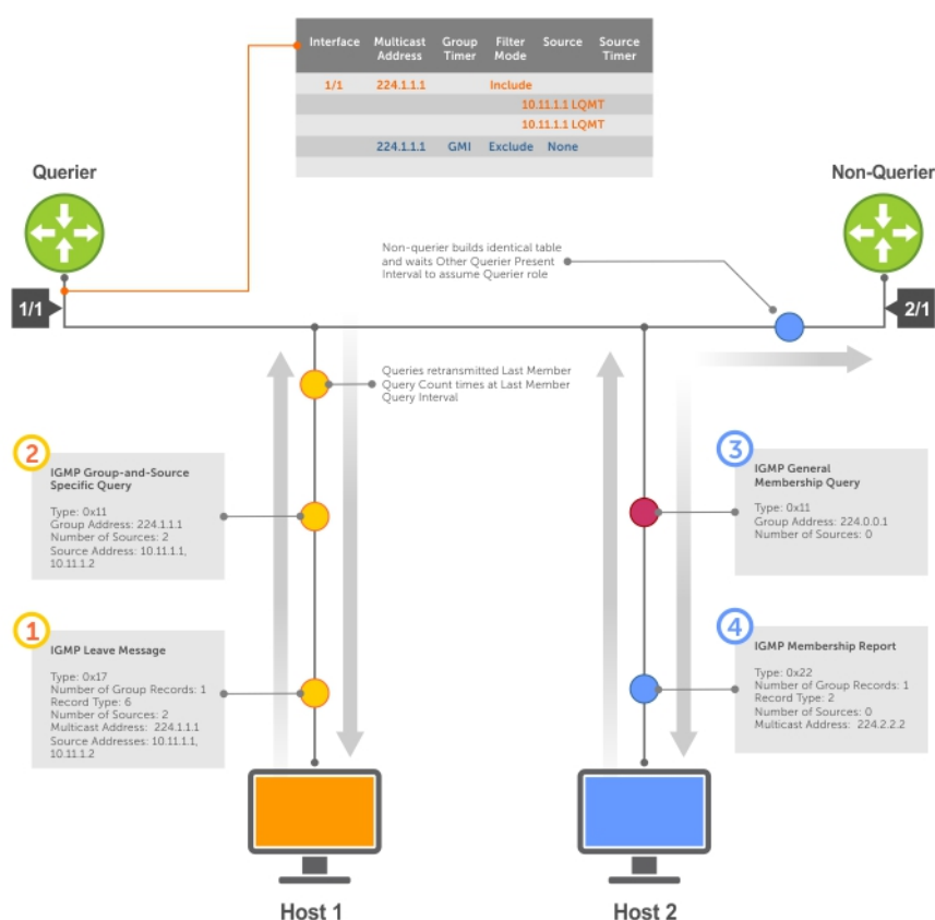
Figure 47. Membership Queries: Leaving and Staying
