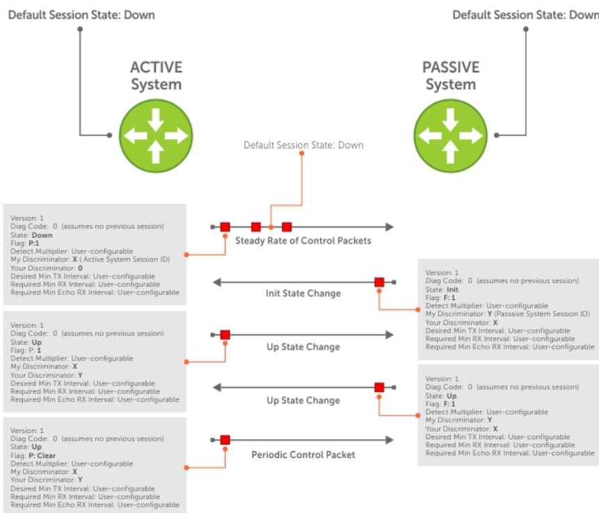
Figure 10. BFD Three-Way Handshake State Changes
