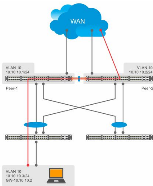
Figure 137. Packets without peer routing enabled
