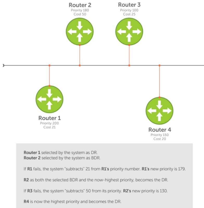
Figure 98. Priority and Cost Examples
