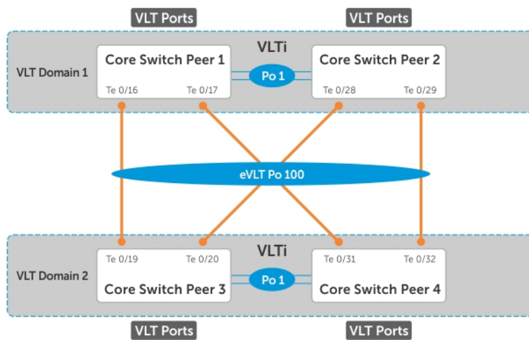
Figure 140. eVLT Configuration Example
