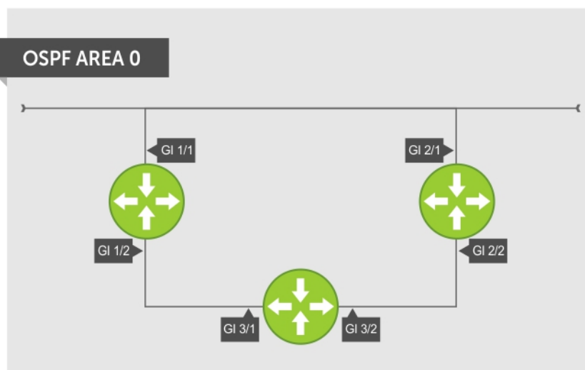
Figure 99. Basic Topology and CLI Commands for OSPFv2
