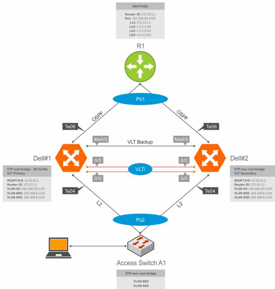
Figure 139. Peer Routing Configuration Example
