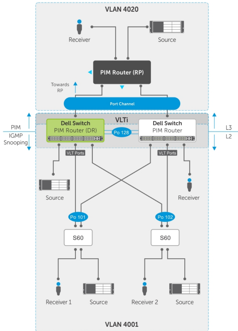
Figure 136. PIM-Sparse Mode Support on VLT
