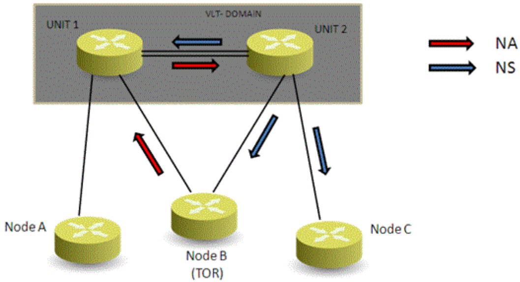
Figure 141. Sample Configuration of IPv6 Peer Routing in a VLT Domain
