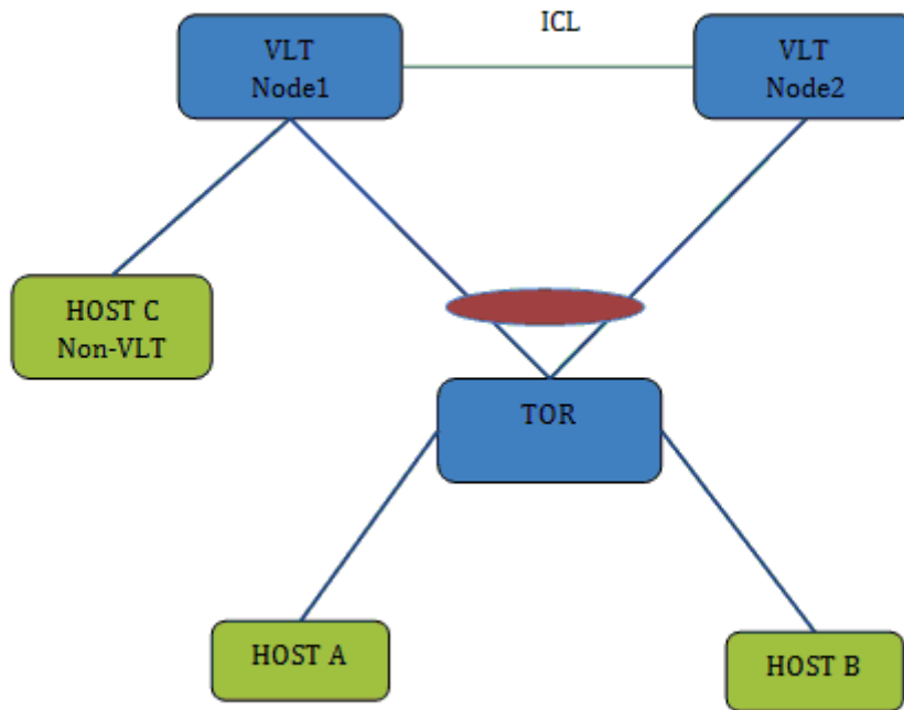
Figure 142. Sample Configuration of IPv6 Peer Routing in a VLT Domain
