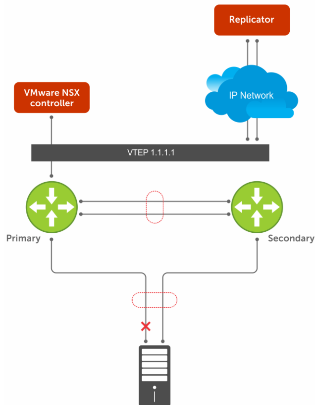
Figure 159. Controller-based VXLAN for VLT Providing Redundancy
