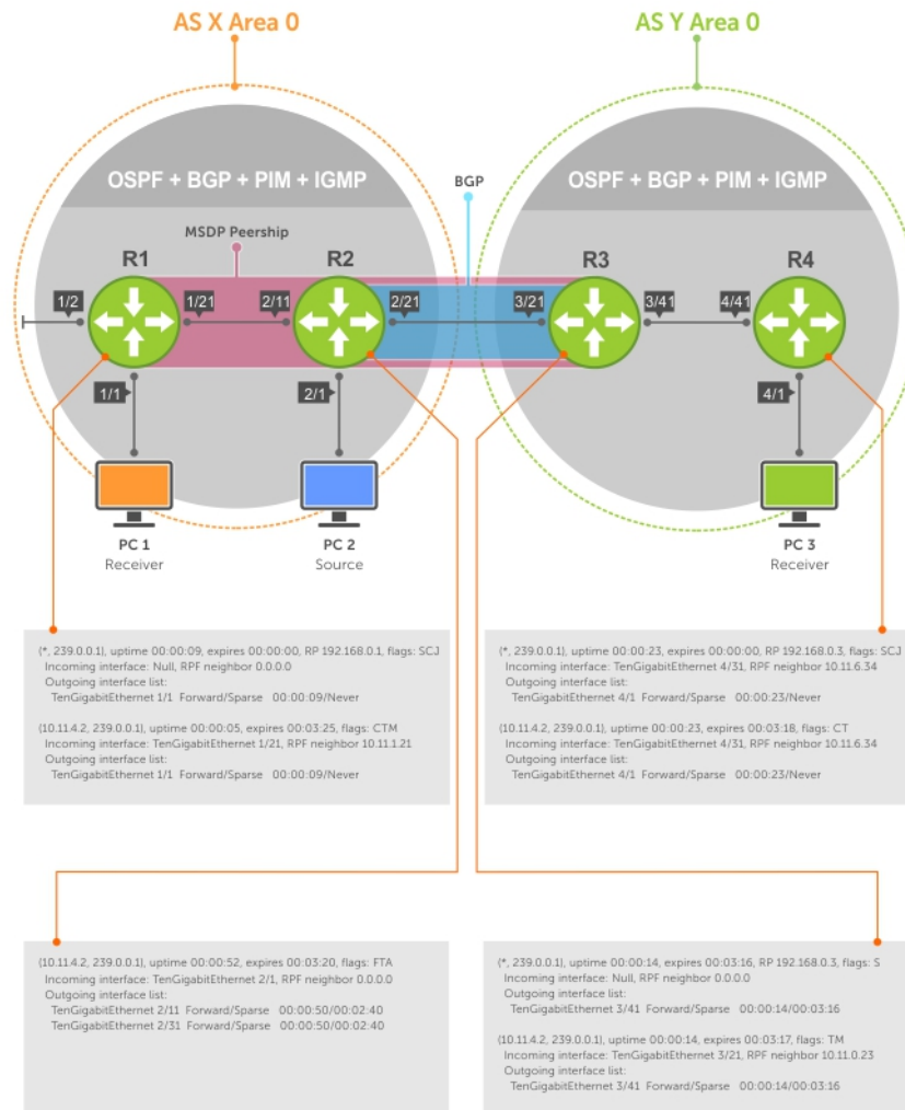
Figure 90. MSDP with Anycast RP
