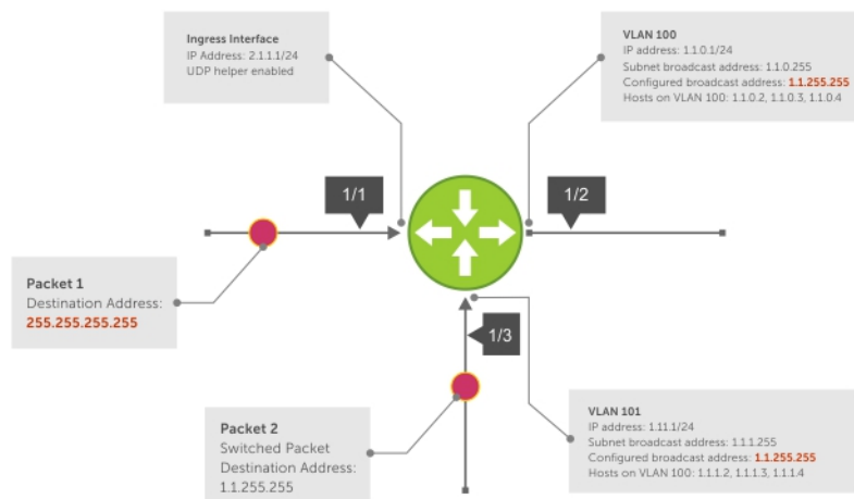
Figure 58. UDP Helper with Configured Broadcast Addresses
