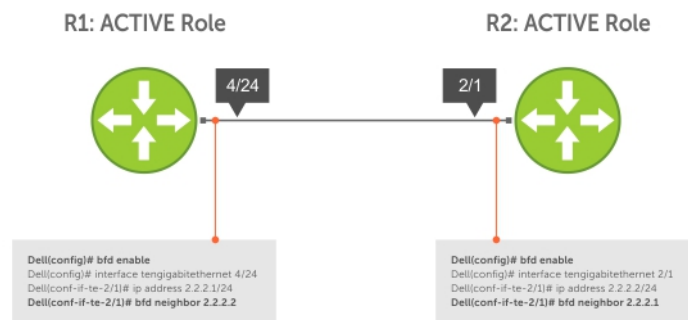
Figure 14. Establishing a BFD Session on Physical Ports
