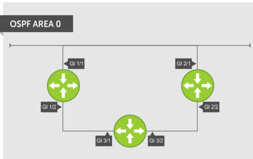
Figure 100. Basic Topology and CLI Commands for OSPFv2
