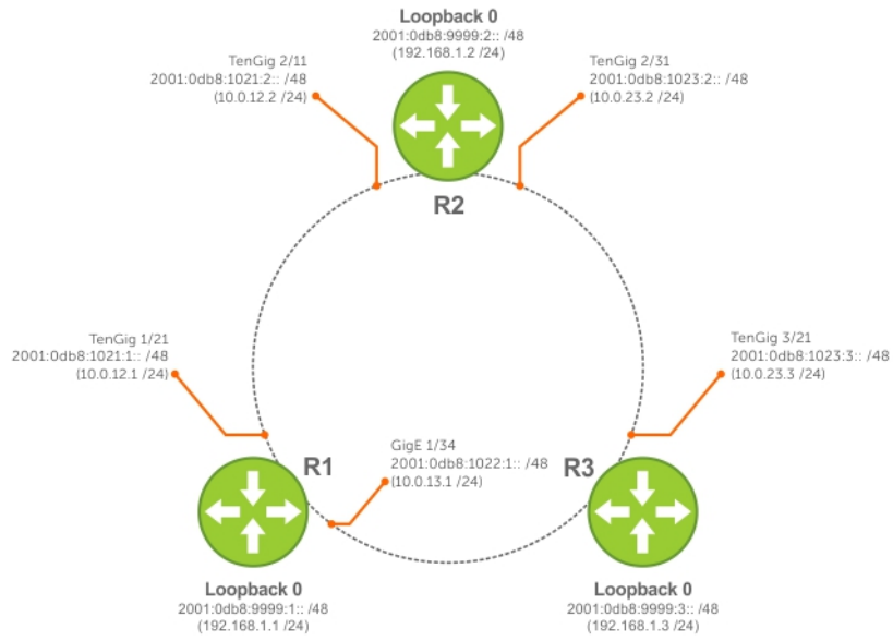
Figure 60. IPv6 IS-IS Sample Topography
