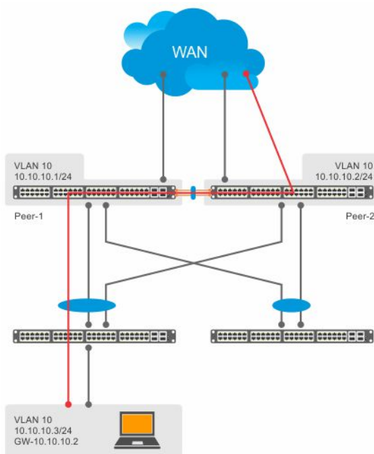
Figure 138. Packets without peer routing enabled
