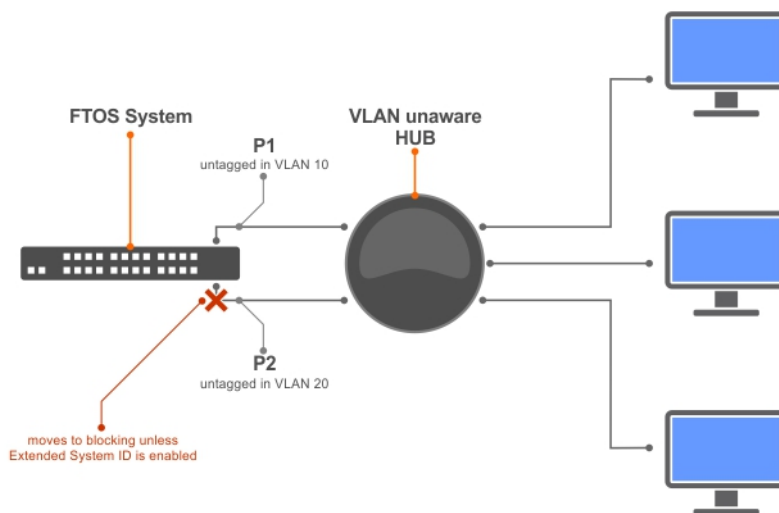
Figure 108. PVST+ with Extend System ID
