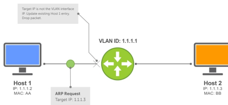
Figure 49. ARP Learning via ARP Request
