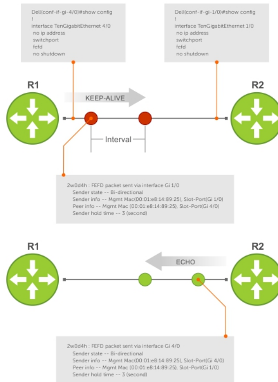
Figure 73. Configuring Far-End Failure Detection
