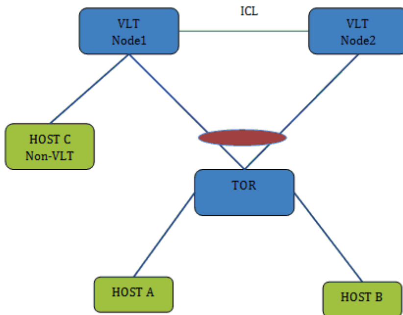
Figure 143. Sample Configuration of IPv6 Peer Routing in a VLT Domain
