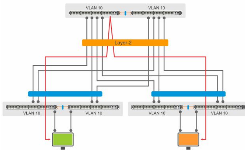
Figure 134. Layer-2 Traffic in VLT Domains
