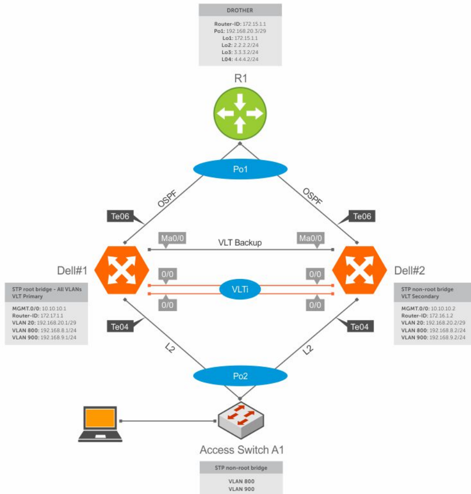
Figure 140. Peer Routing Configuration Example
