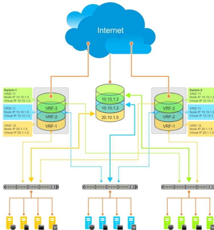
Figure 174. VRRP in a VRF: Non-VLAN Example
