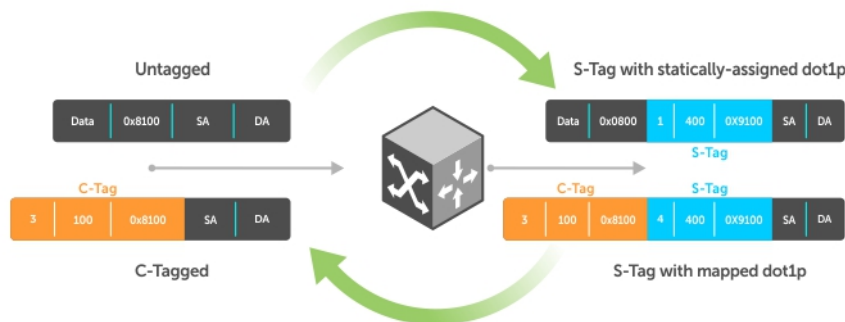
Figure 118. Statically and Dynamically Assigned dot1p for VLAN Stacking
