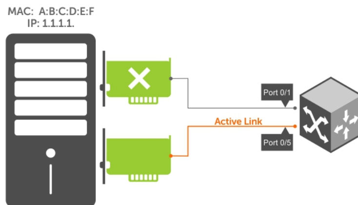
Figure 70. Redundant NICs with NIC Teaming
