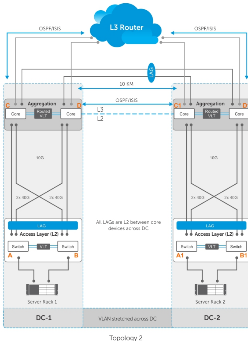
Figure 145. Sample Configuration for a VLT Proxy Gateway
