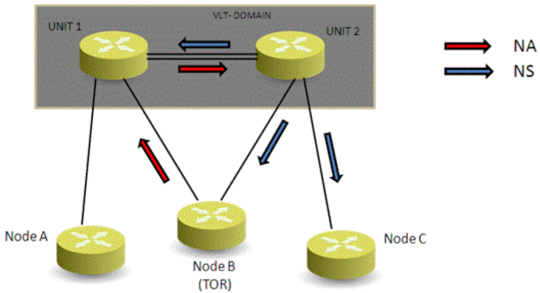
Figure 142. Sample Configuration of IPv6 Peer Routing in a VLT Domain
