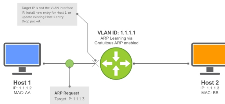
Figure 55. ARP Learning via ARP Request with ARP Learning via Gratuitous ARP Enabled
