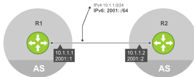
Figure 29. Configure IPv6 NH to advertise IPv6 prefix over IPv4 neighbor
