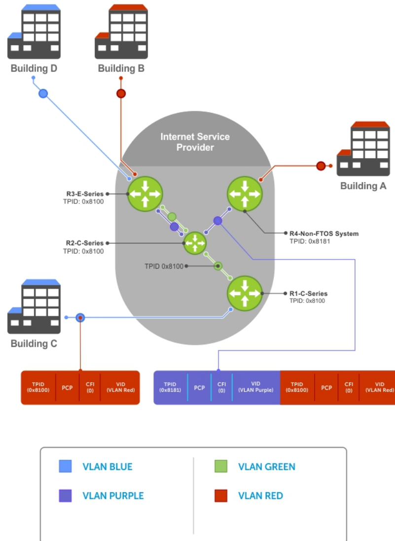
Figure 117. Single and Double-Tag TPID Match
