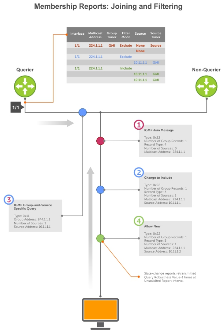
Figure 48. Membership Reports: Joining and Filtering
