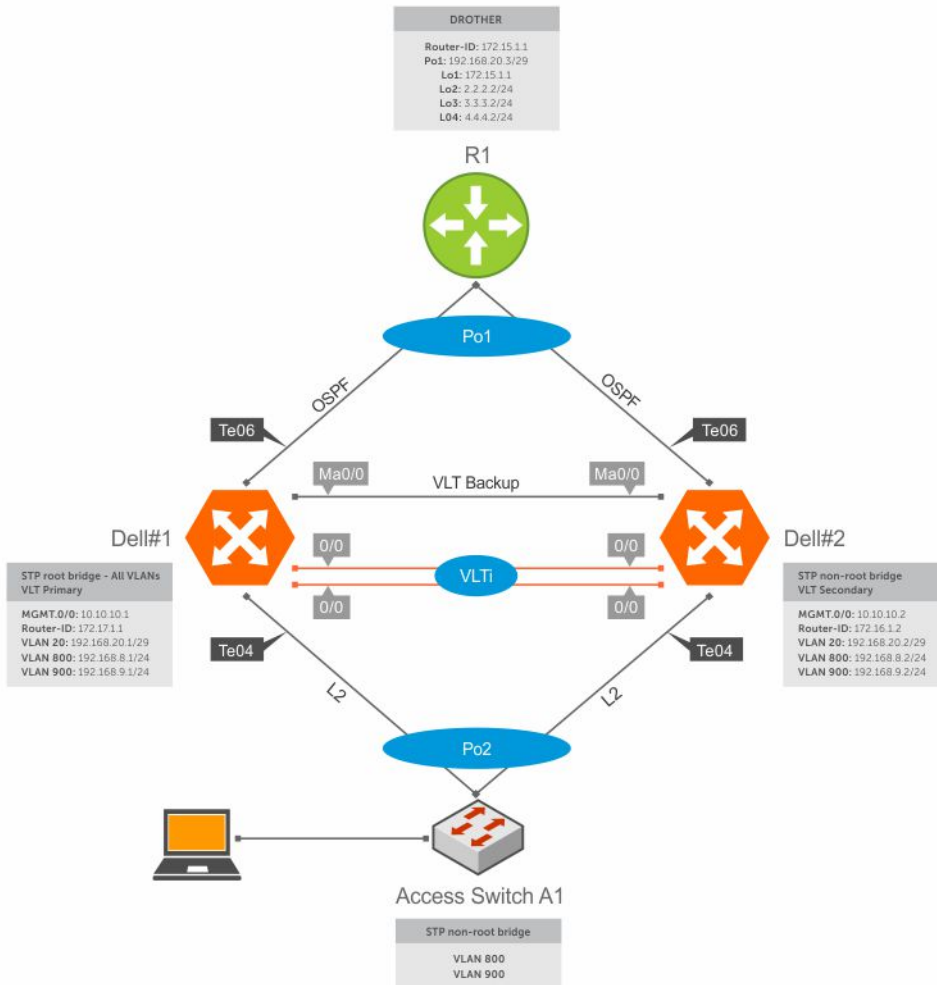
Figure 145. Peer Routing Configuration Example
