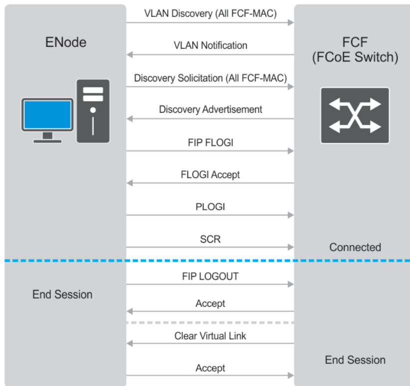
Figure 38. FIP Discovery and Login Between an ENode and an FCF
