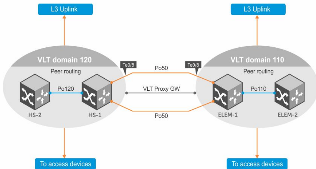
Figure 151. VLT Proxy Gateway Sample Topology
