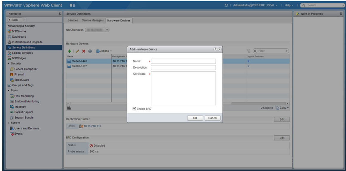
Figure 154. Create VXLAN Gateway
