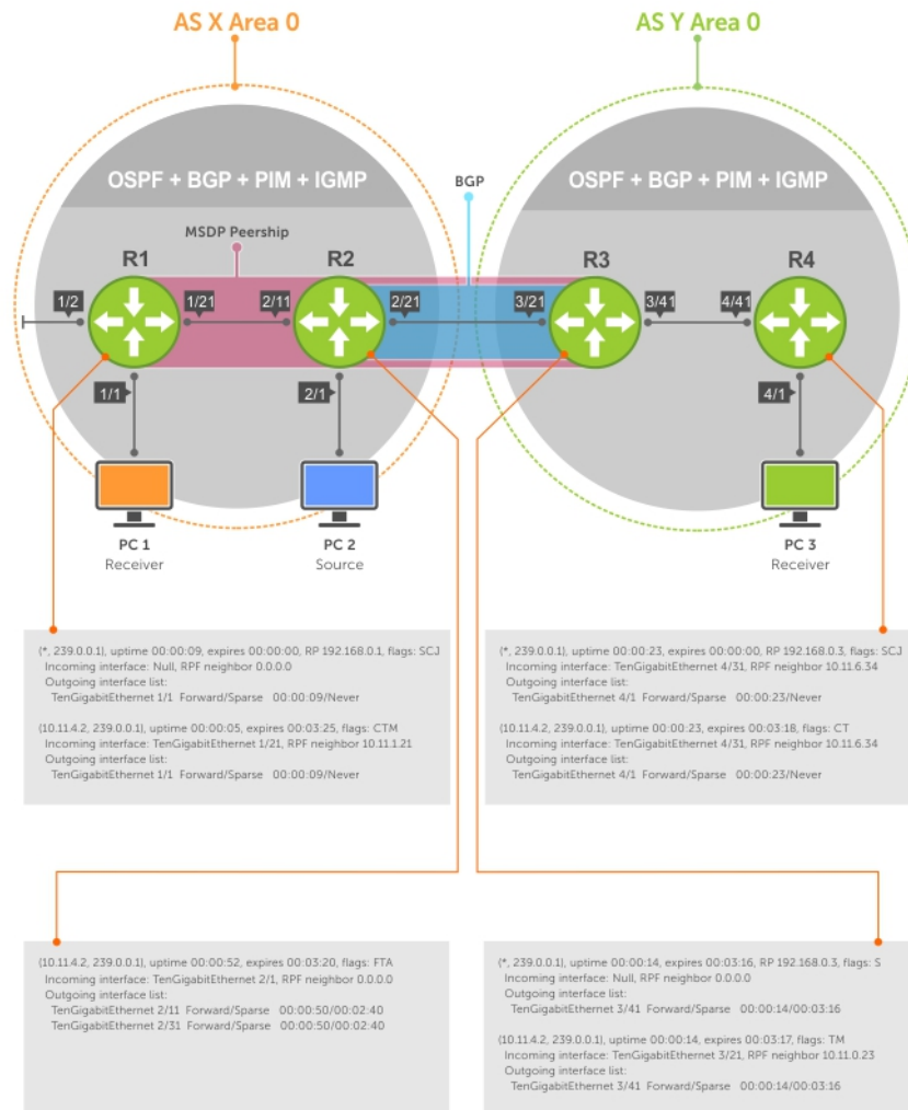
Figure 93. MSDP with Anycast RP
