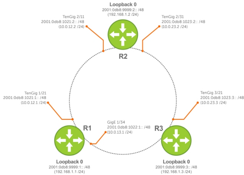
Figure 62. IPv6 IS-IS Sample Topography
