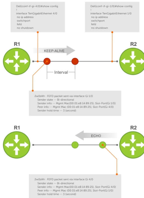
Figure 75. Configuring Far-End Failure Detection
