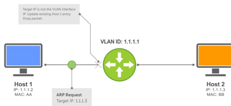
Figure 51. ARP Learning via ARP Request
