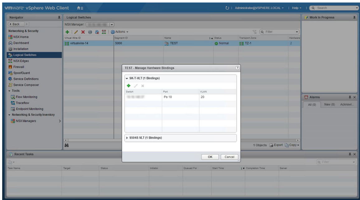
Figure 159. Create Logical Switch Port
