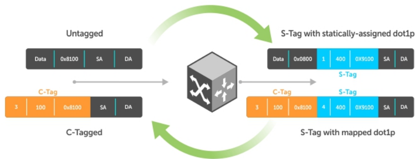
Figure 120. Statically and Dynamically Assigned dot1p for VLAN Stacking
