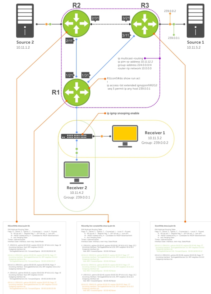
Figure 97. Preventing a Source from Transmitting to a Group
