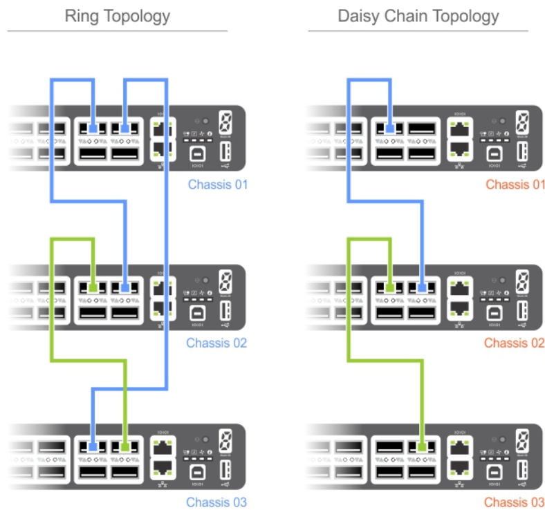
Figure 123. Supported Stacking Topologies
