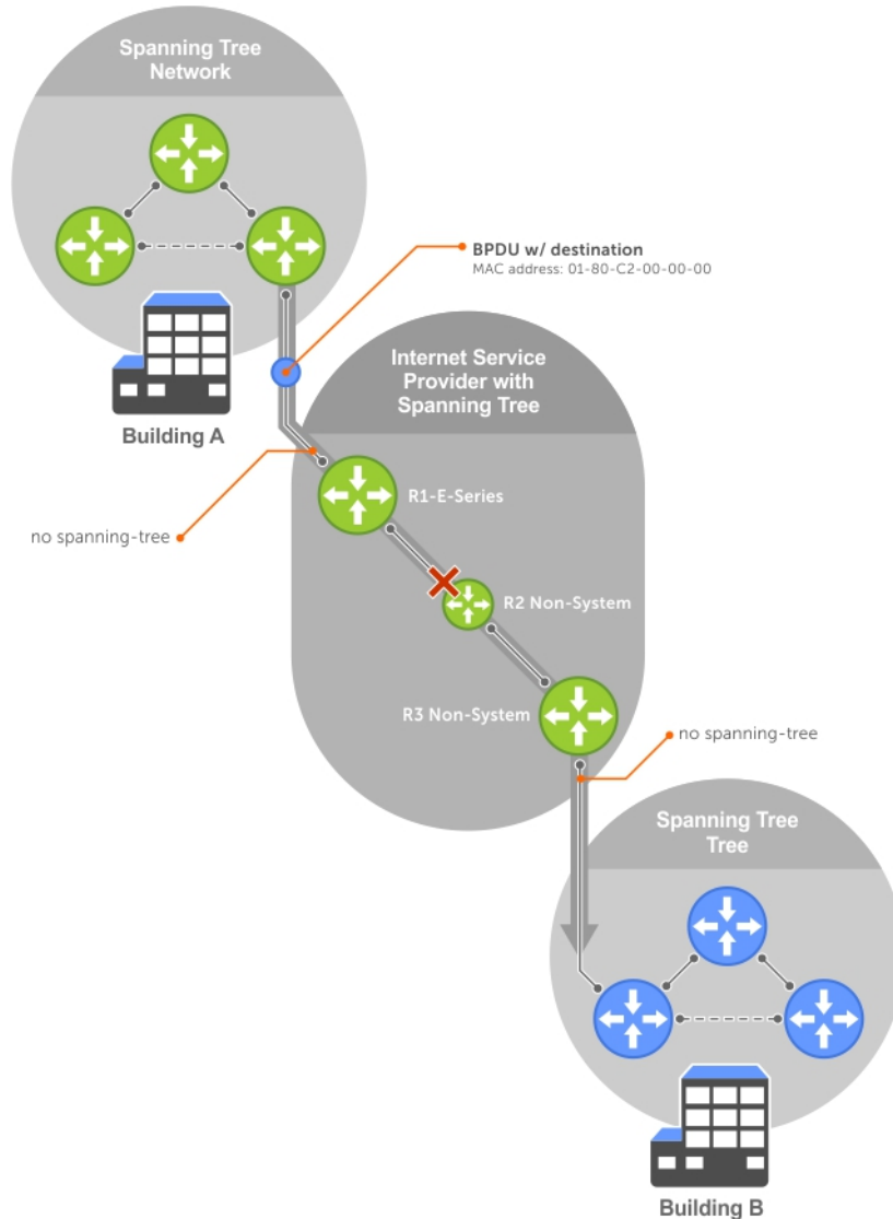
Figure 121. VLAN Stacking without L2PT
