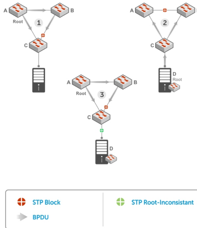
Figure 129. STP Root Guard Prevents Bridging Loops
