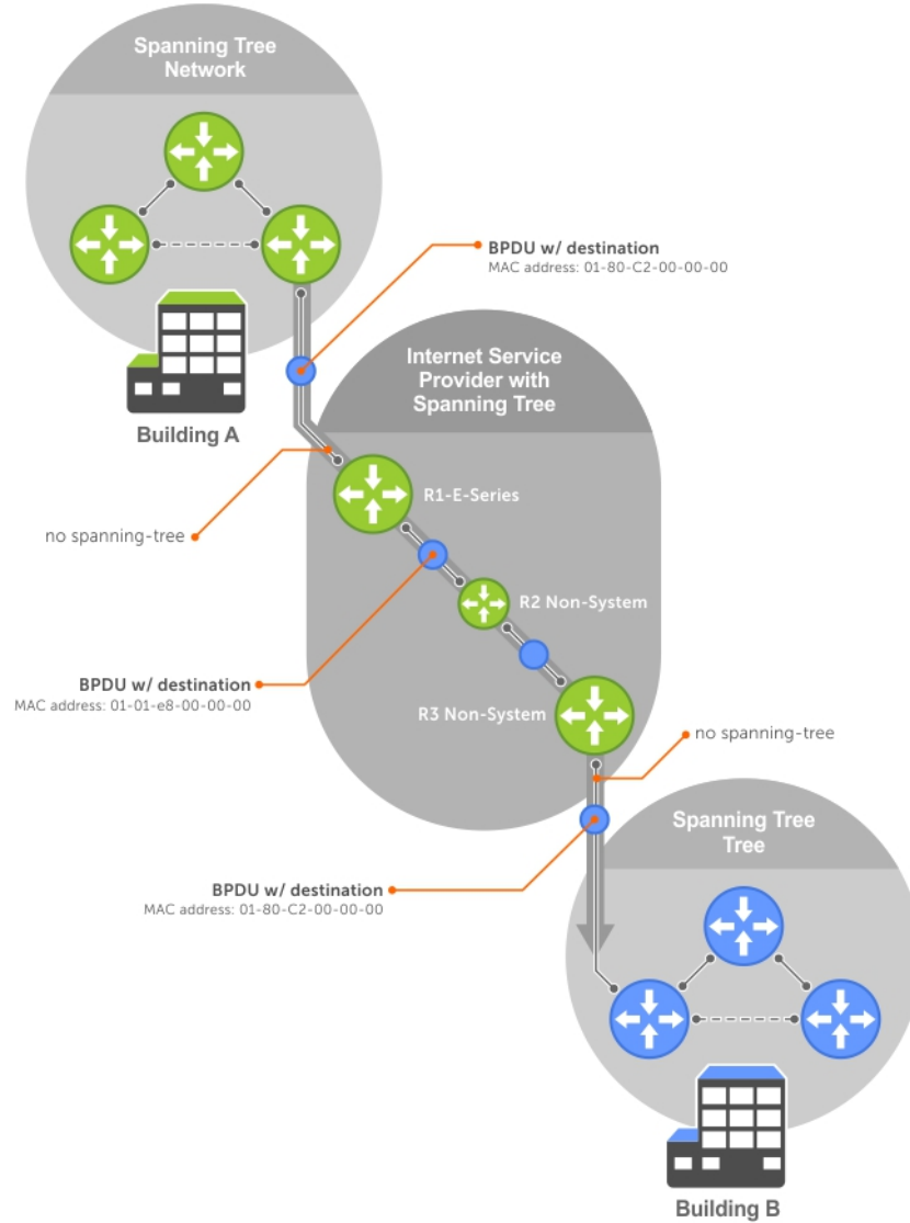
Figure 122. VLAN Stacking with L2PT
