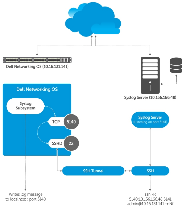
Figure 2. Setting Up a Secure Connection to a Syslog Server
