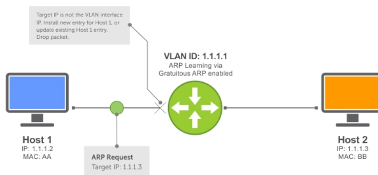
Figure 54. ARP Learning via ARP Request with ARP Learning via Gratuitous ARP Enabled
