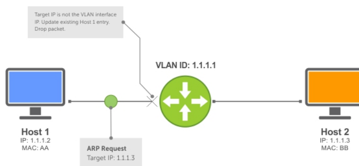
Figure 53. ARP Learning via ARP Request
