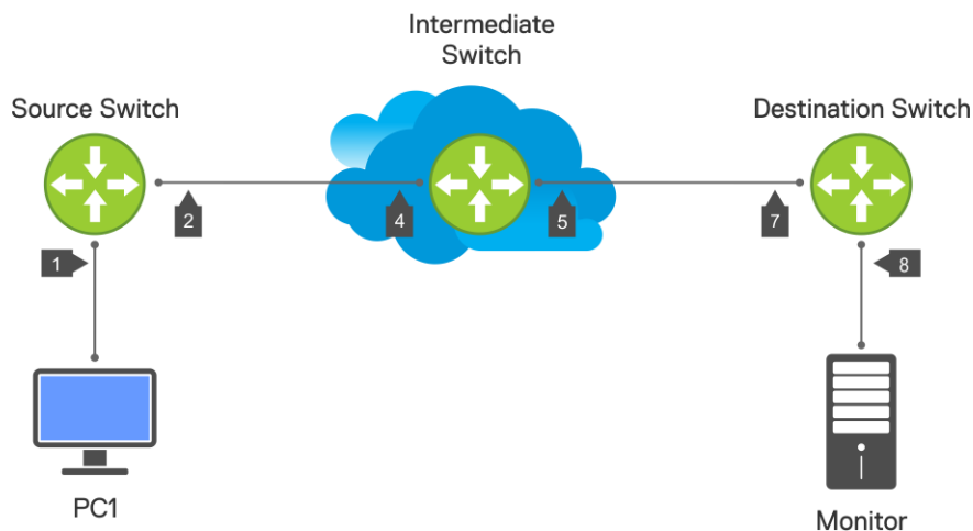
Figure 108. RPM Configuration
