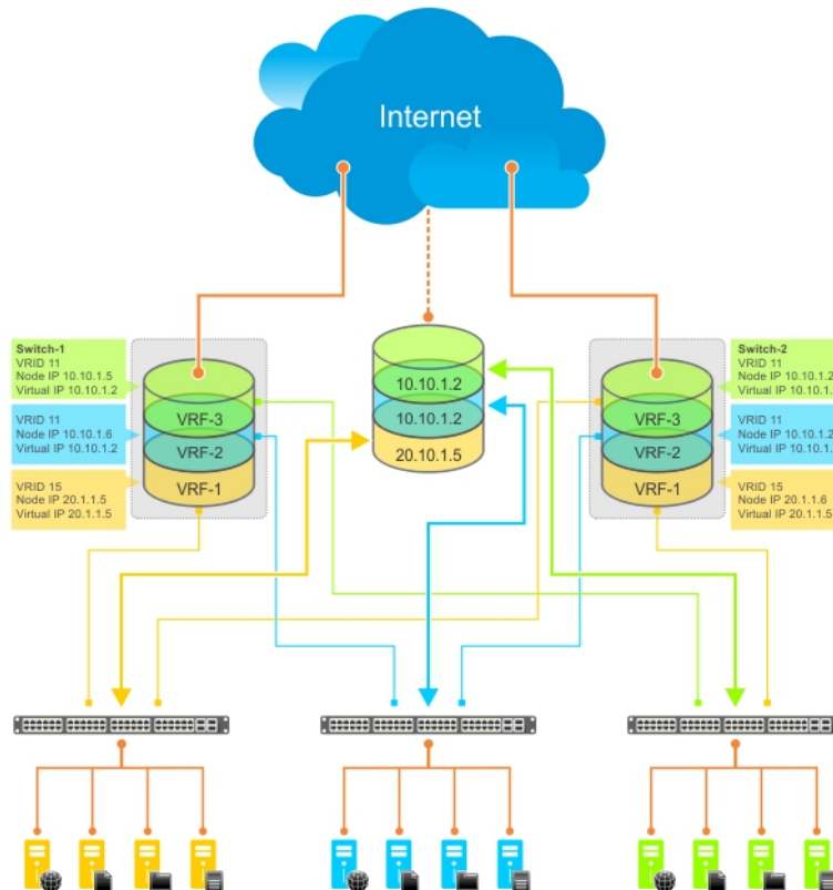
Figure 182. VRRP in a VRF: Non-VLAN Example
