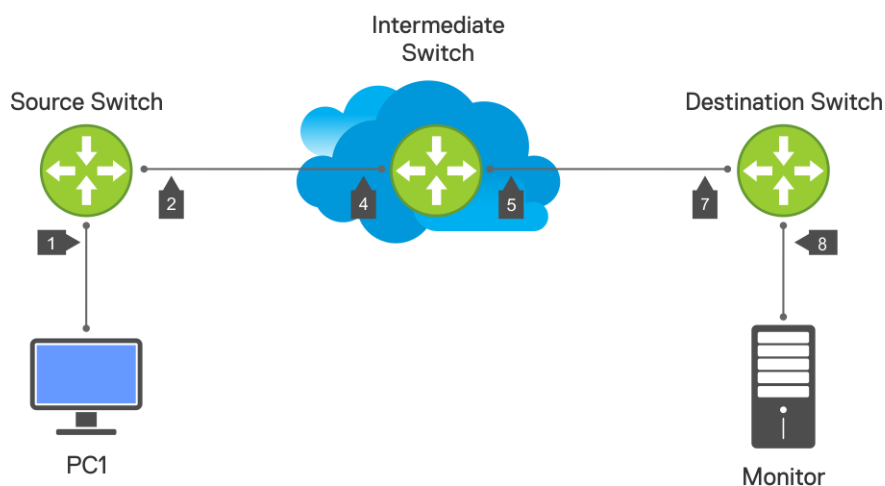
Figure 108. RPM Configuration
