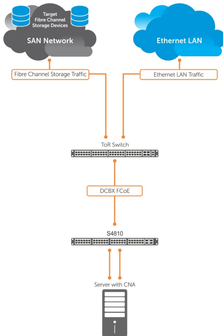
Figure 40. FIP Snooping on a Dell EMC Networking Switch
