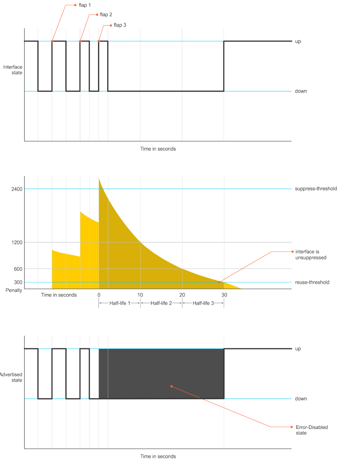
Figure 52. Interface State Change
