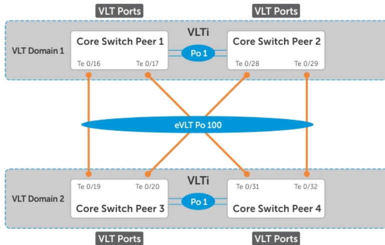
Figure 149. eVLT Configuration Example
