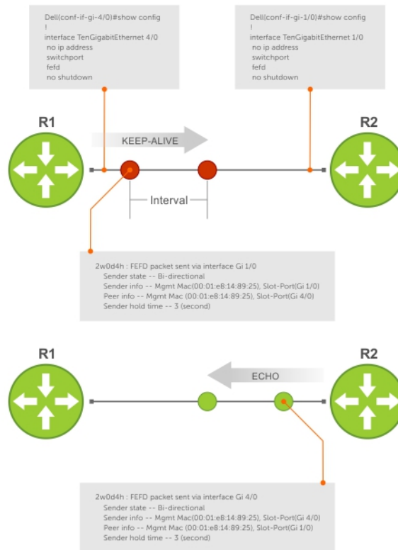
Figure 77. Configuring Far-End Failure Detection
