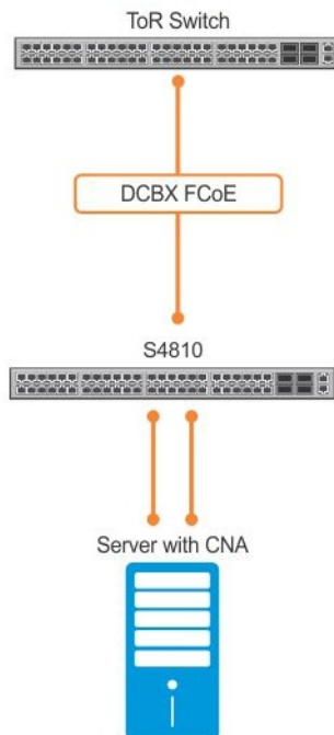
Figure 41. Configuration Example: FIP Snooping on a Switch
