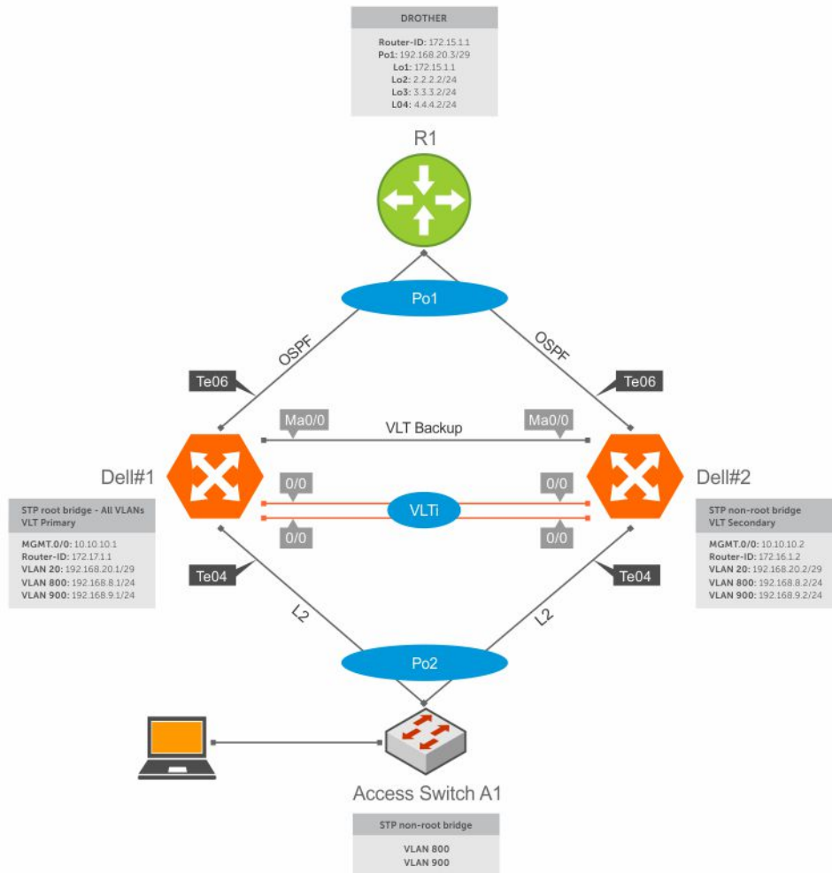
Figure 148. Peer Routing Configuration Example
