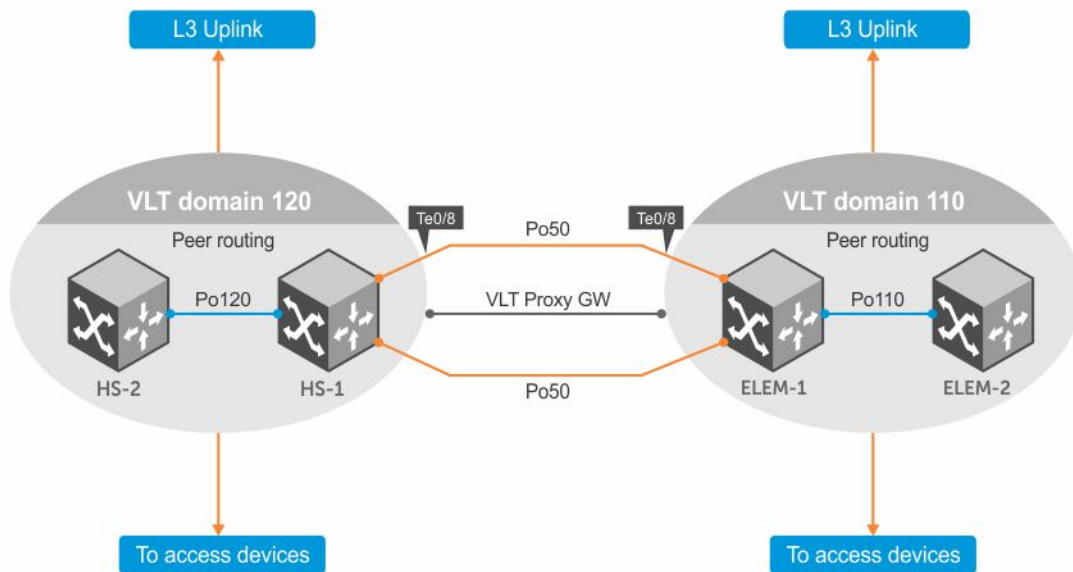
Figure 154. VLT Proxy Gateway Sample Topology
