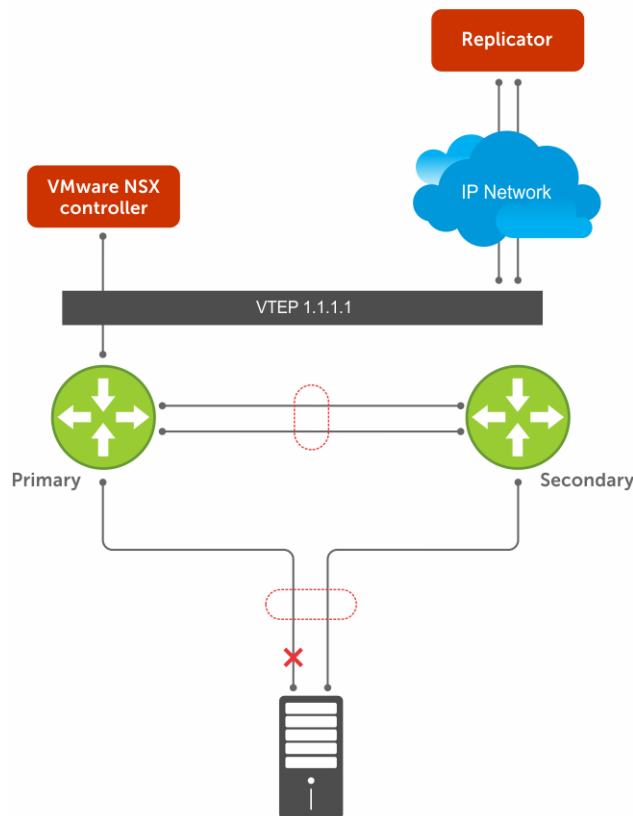
Figure 168. Controller-based VXLAN for VLT Providing Redundancy
