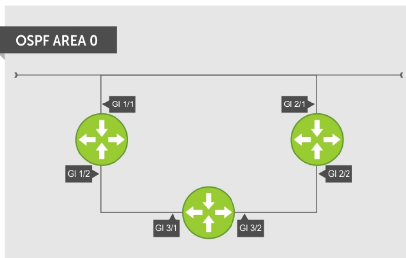
Figure 104. Basic Topology and CLI Commands for OSPFv2
