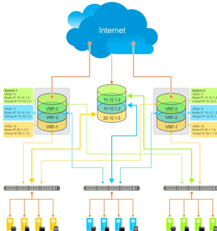
Figure 175. VRRP in a VRF: Non-VLAN Example
