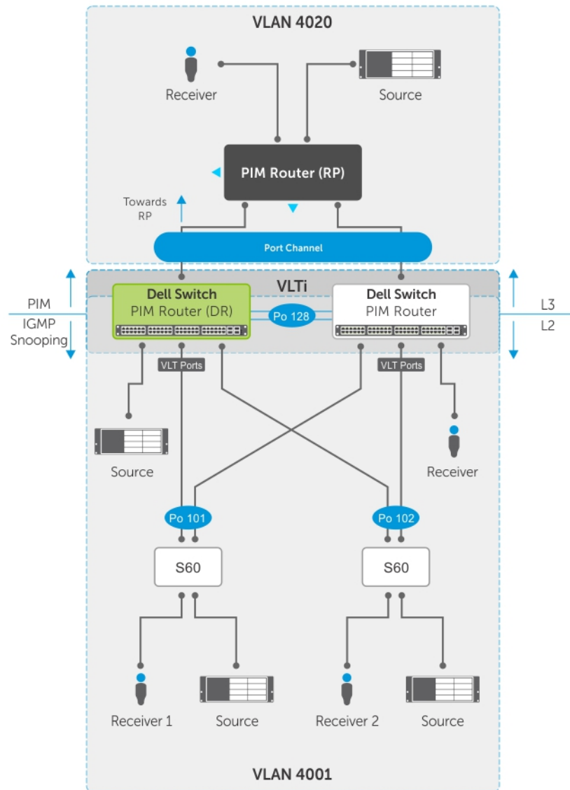
Figure 145. PIM-Sparse Mode Support on VLT
