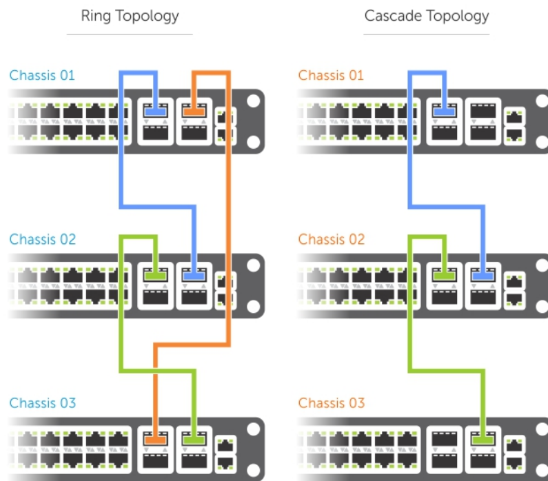
Figure 126. Supported Stacking Topologies
