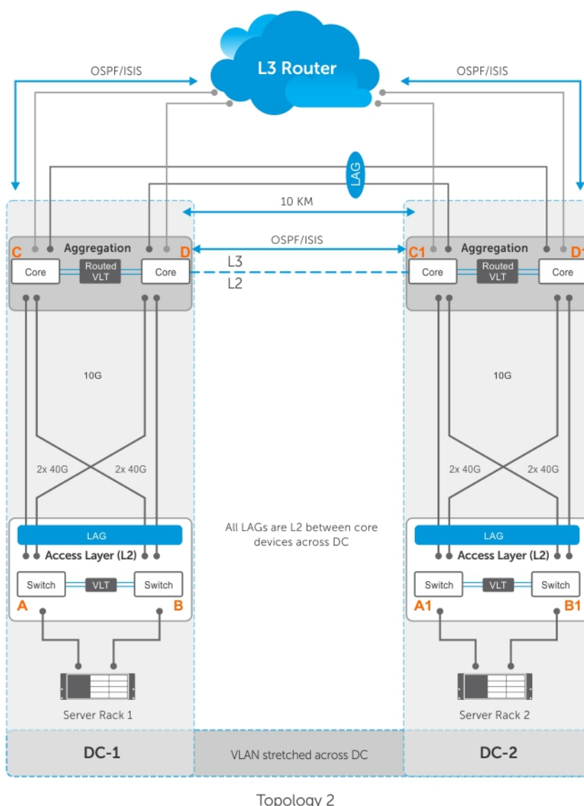
Figure 153. Sample Configuration for a VLT Proxy Gateway
