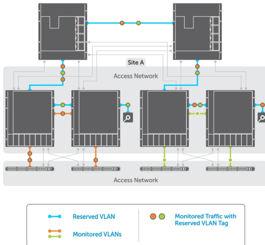
Figure 107. Remote Port Mirroring
