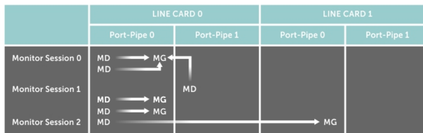
Figure 105. Port Monitoring Configurations
