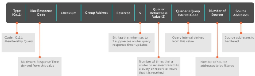
Figure 47. IGMP Version 3 Packet Structure
