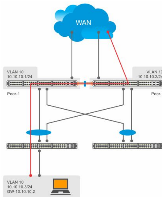
Figure 146. Packets without peer routing enabled
