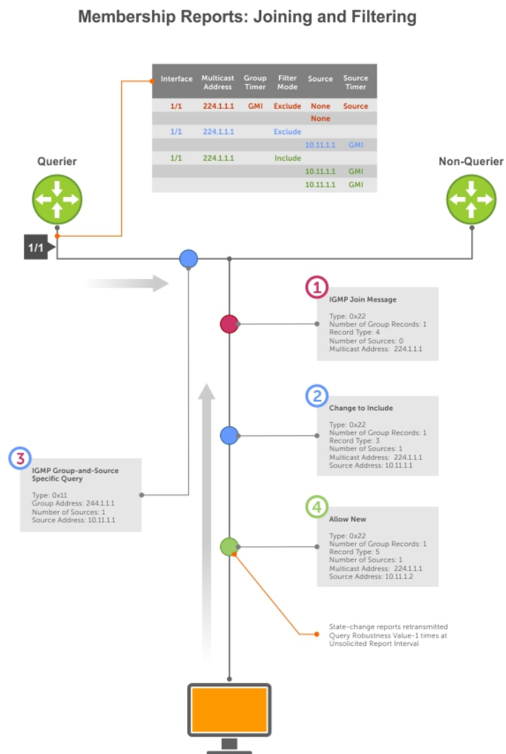
Figure 49. Membership Reports: Joining and Filtering
