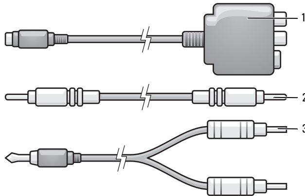
1 TV/digital audio adapter 2 composite video cable 3 standard audio cable
