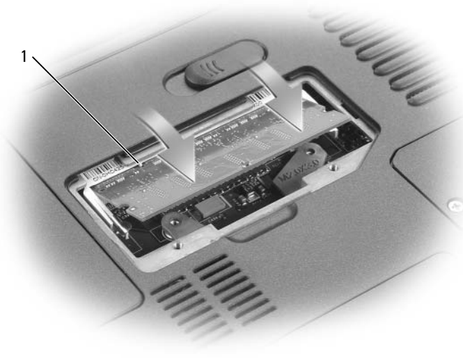
1 tab in connector slot
