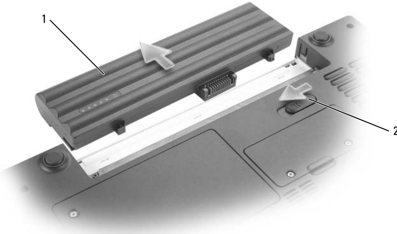
1 battery 2 battery-bay latch release
