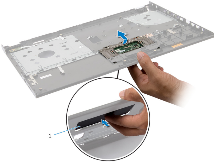
1 touch pad
