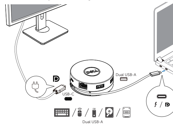
With Power Delivery Pass-Through Via USB-C Monitor
