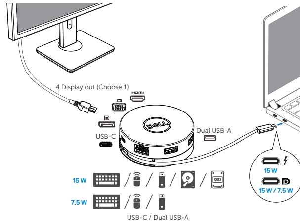
Without Power Delivery Pass-Through
