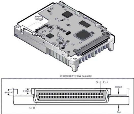
Figure 1. Interface connector
