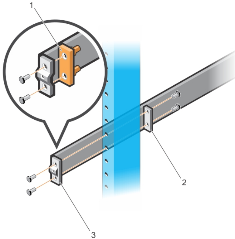
Figure 12. Two-post flush-mount installation
