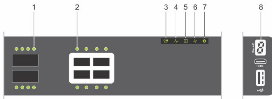
Figure 6. S4128F-ON I/O-side LEDs
