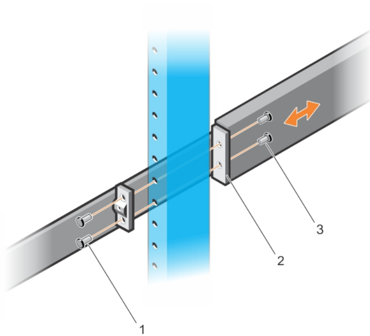
Figure 13. Two-post center-mount installation
