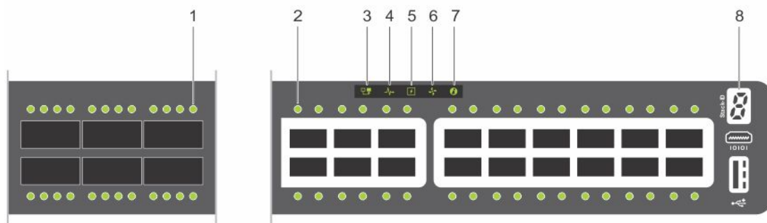
Figure 7. S4148F-ON and S4148FE-ON I/O-side LEDs
