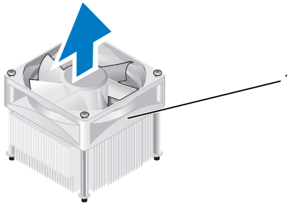
1 processor fan/heat sink assembly
