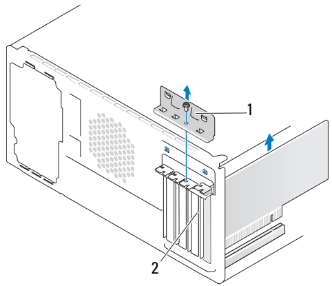
1 card retention bracket 2 filler bracket
