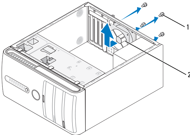
1 screws (4) 2 chassis fan
