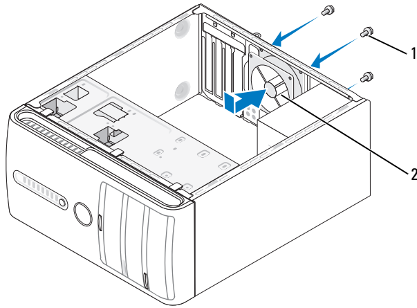
1 screws (4) 2 chassis fan
