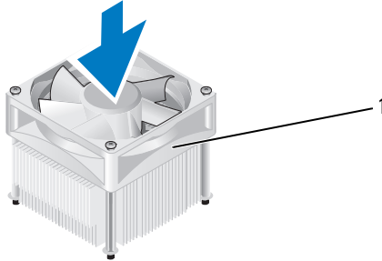
1 processor fan/heat sink assembly
